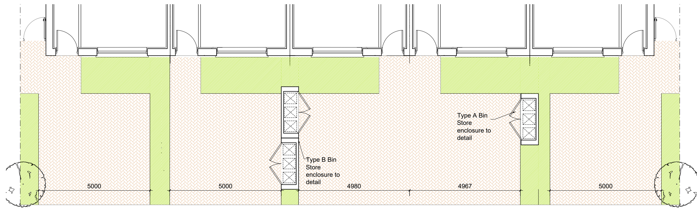
TYPICAL BIN STORE DETAIL 1:100 FOR 5 TERRACE B1-B-B-B-B1
