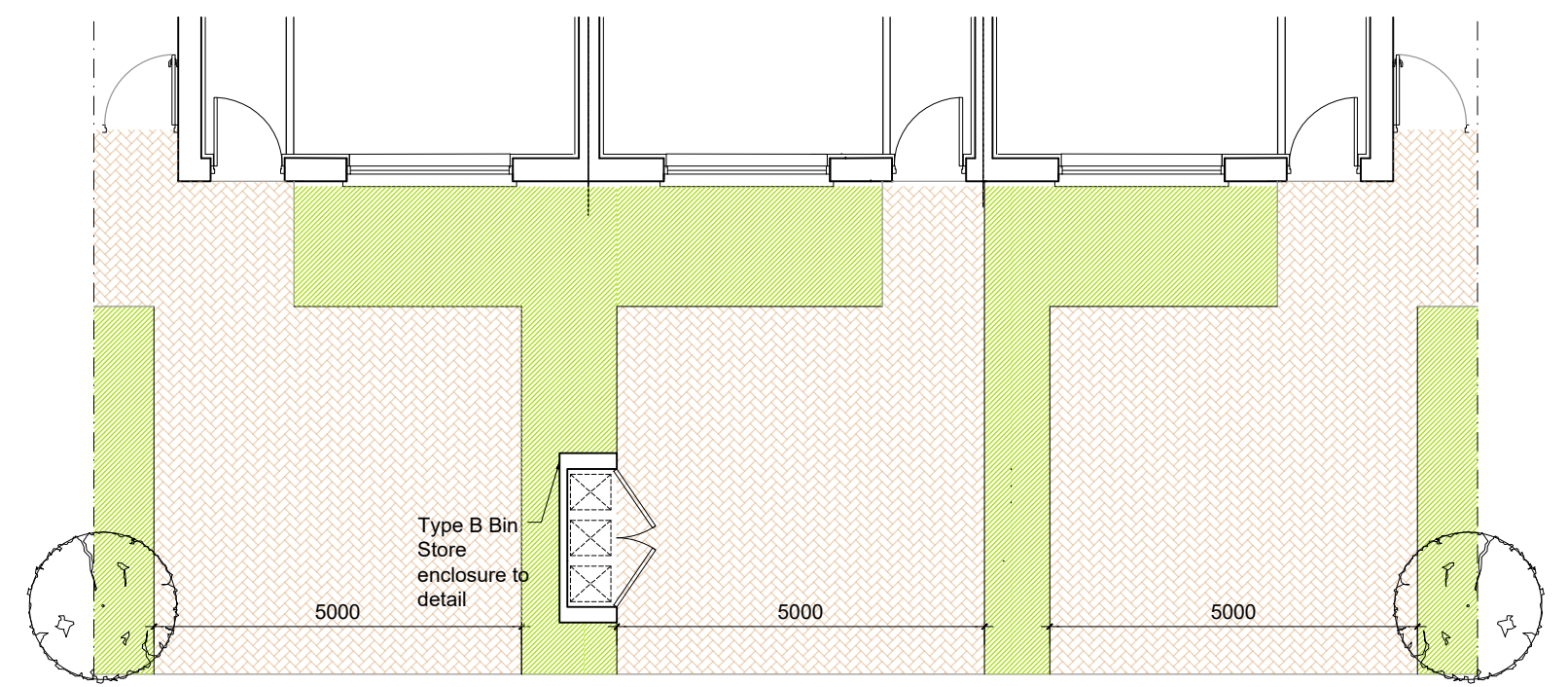
TYPICAL BIN STORE DETAIL 1:100 FOR 3 TERRACE B1-B-B1
