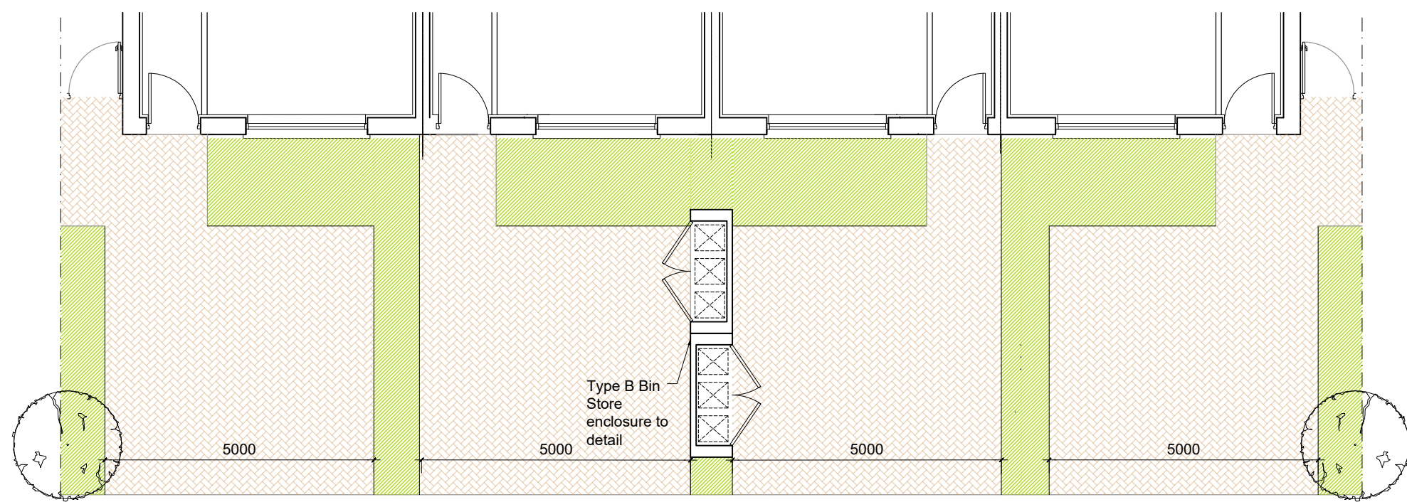
TYPICAL BIN STORE DETAIL 1:100 FOR 4 TERRACE B1-B-B-B1
